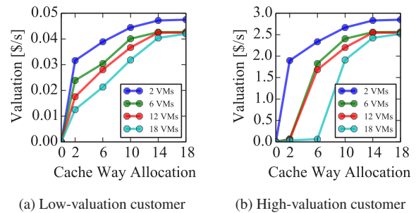
Figure 5: Composite-Scimark valuation function for different server-loads (i.e., active VMs) and when allocated 2 hardware threads. Note the different scale in the vertical axes.
